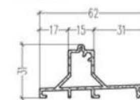
Solera Aluminio 31mm 104.329
